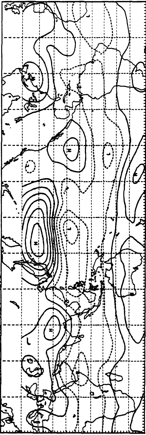
STREAM FUNCTION 200MB NOV 1979
